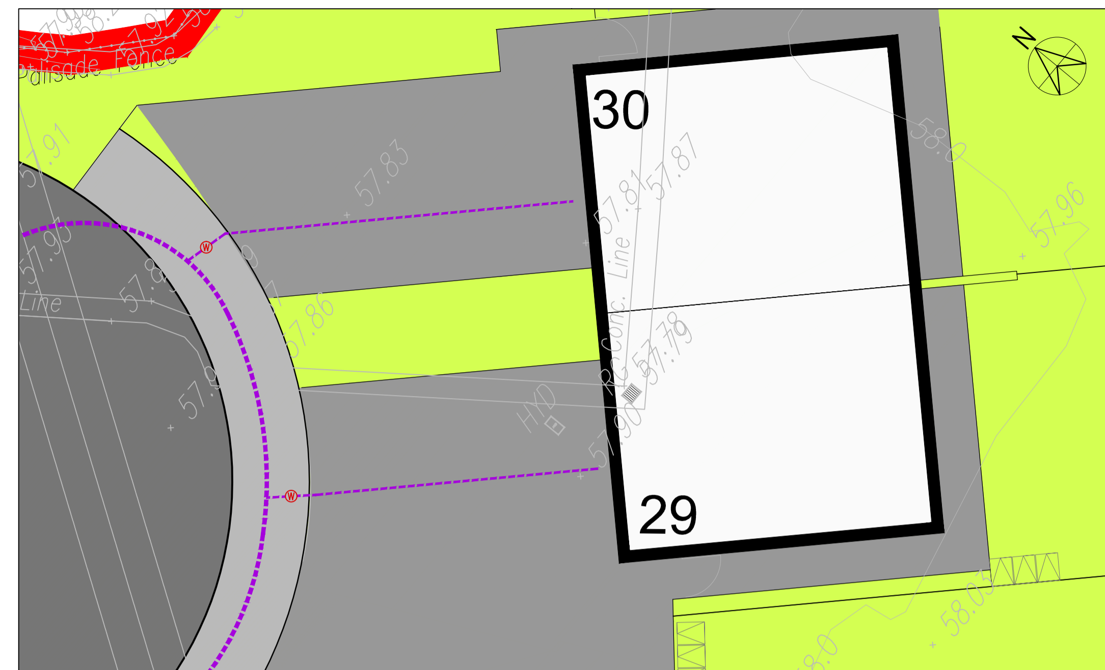
TYPICAL WATERMAIN CONNECTION TO DWELLINGS SHOWING WATER METER SCALE: 1:100
